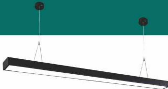
T 9419/6500k 24w L120xW70xH40 LED Giá 698.000đ
