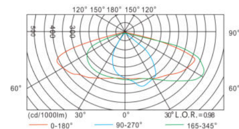
Photometric data
