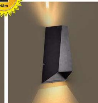
CN-308 L100 x W60 x H175 COB 3W x 2 - Cree USA 810.000đ
